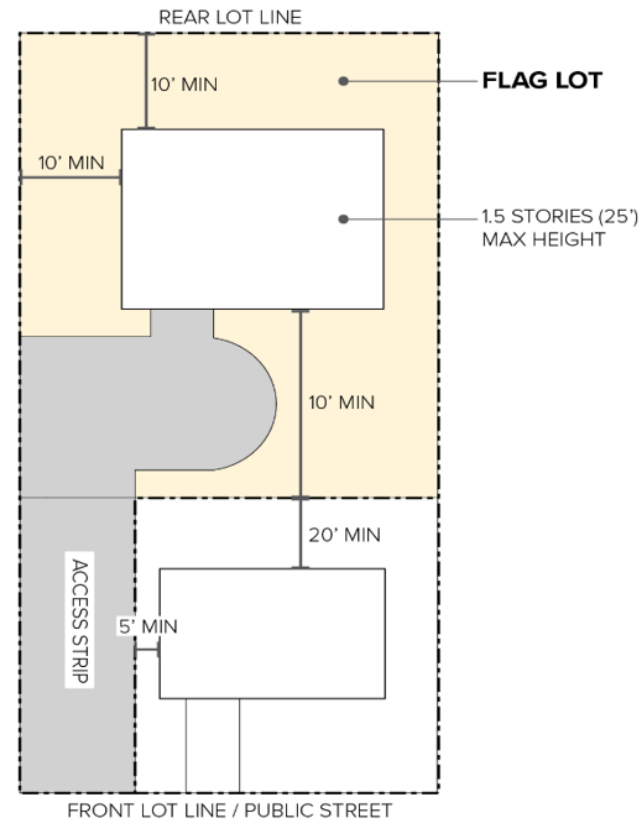
Figure 3. Flag Lot
