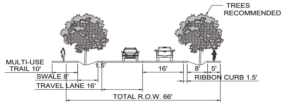
Figure 4. 60' R.O.W.
