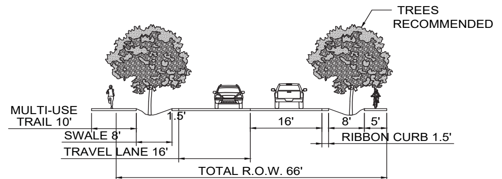
Figure 2. 60' R.O.W.
