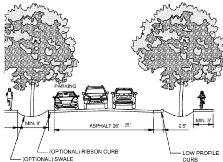
Figure 5. Bioswale
